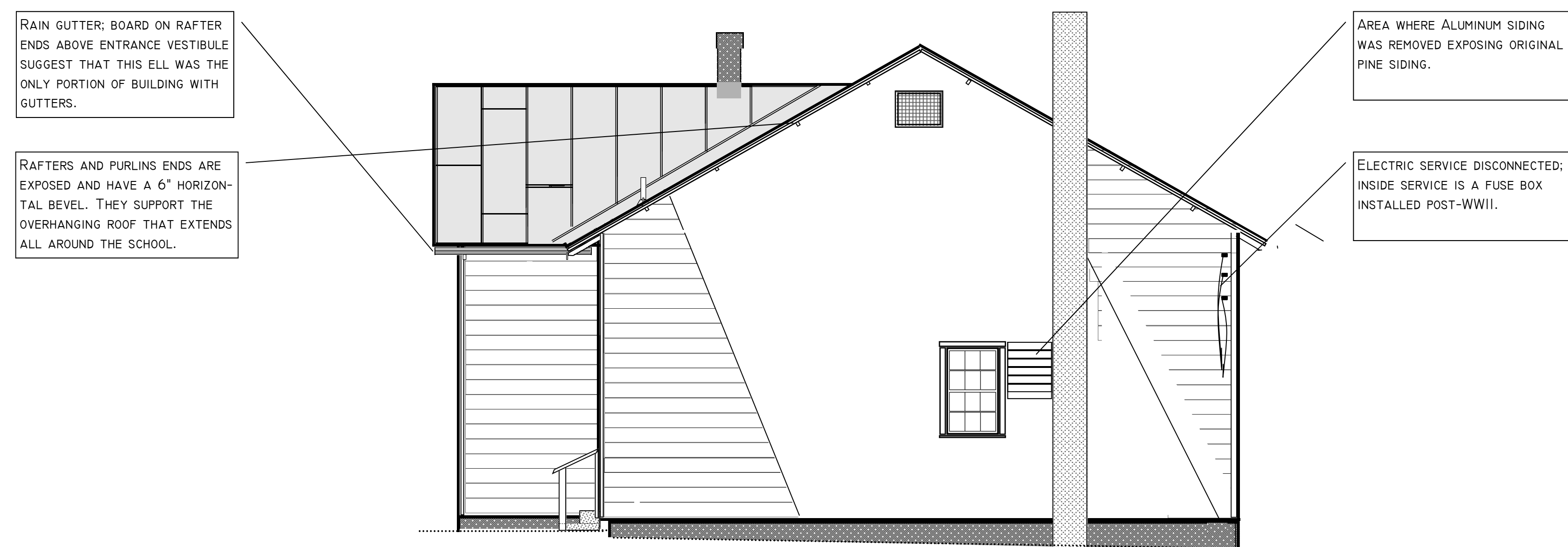
EAST ELEVATION
