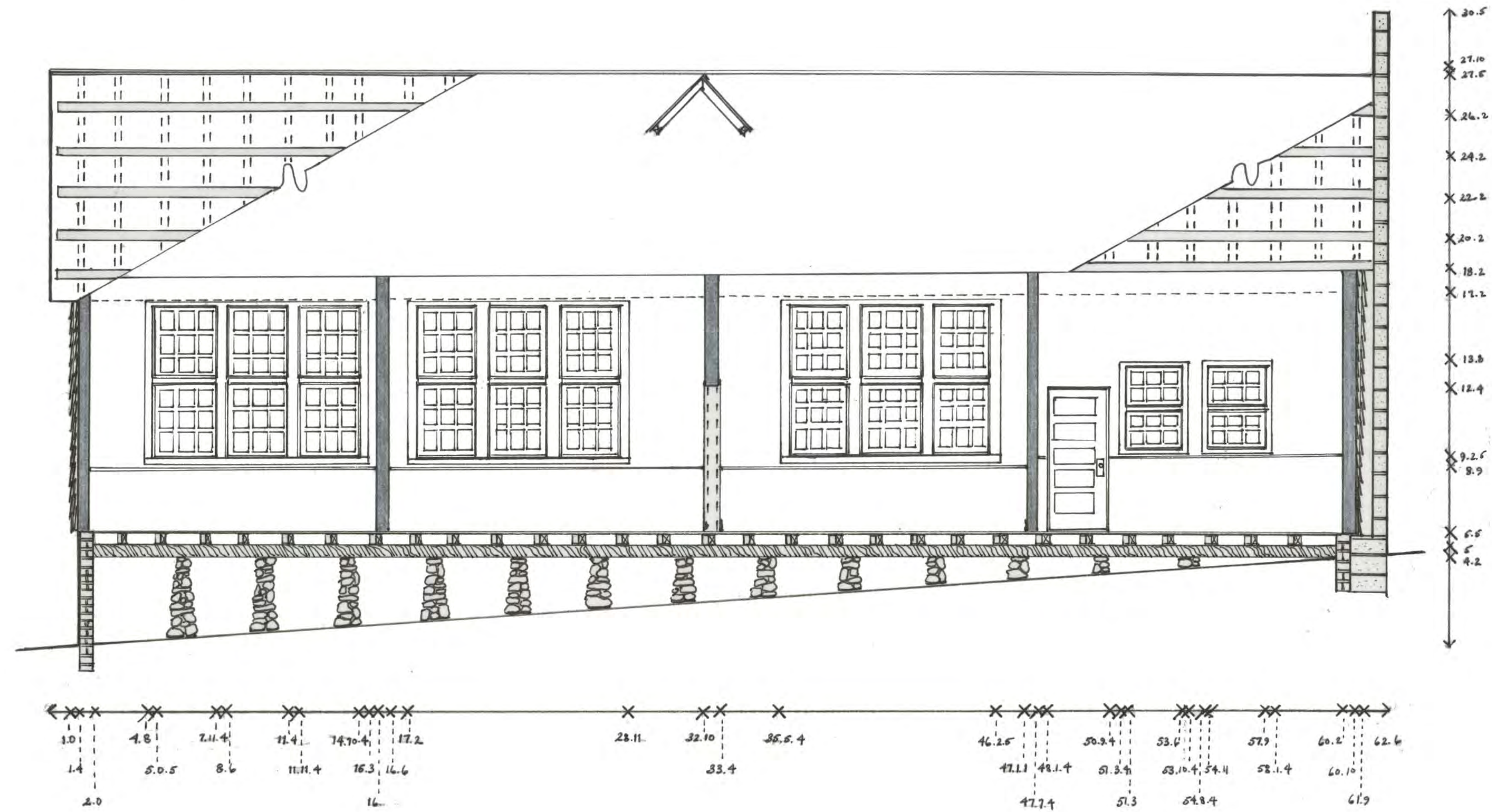
SECTION A - A LONGITUDIONAL SECTION LOOKING EAST 1/4" = 1'
