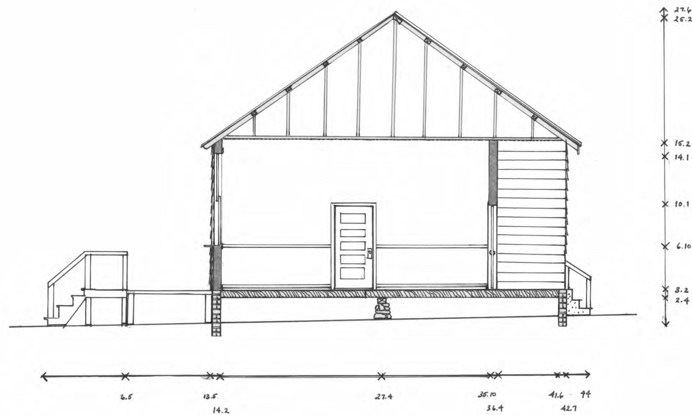
SECTION B - B LATIGUTIONAL SECTION LOOKING SOUTH 1/4" = 1'
