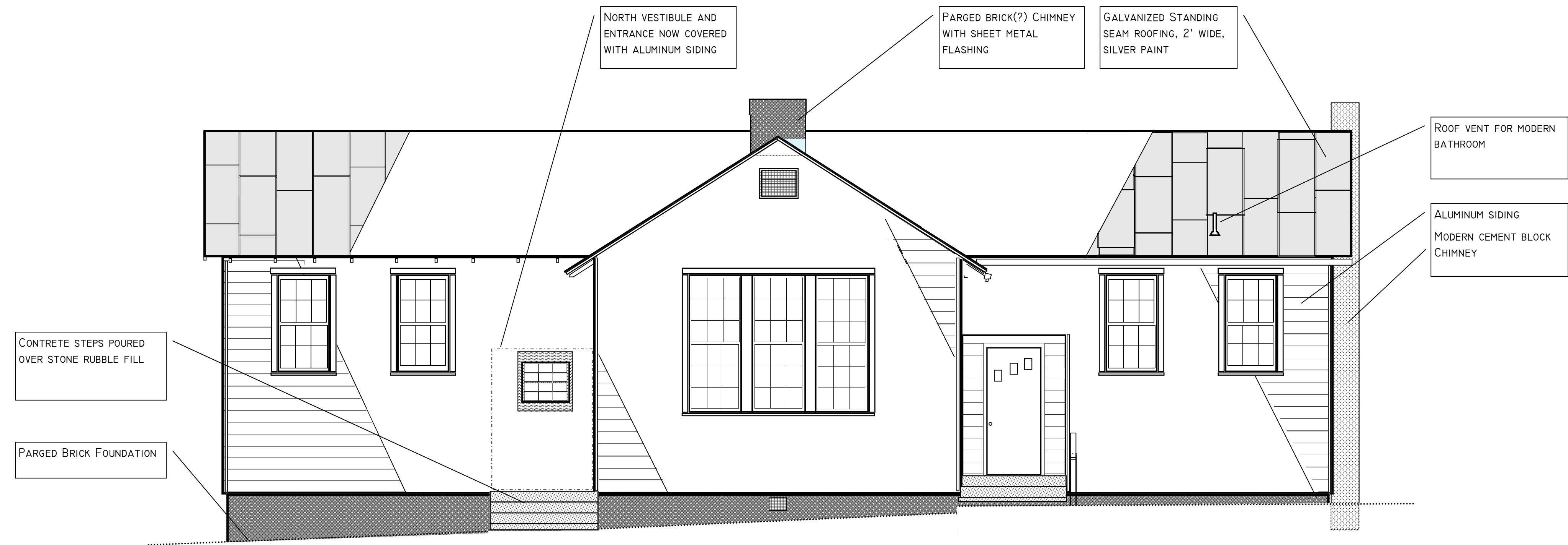
WEST ELEVATION
